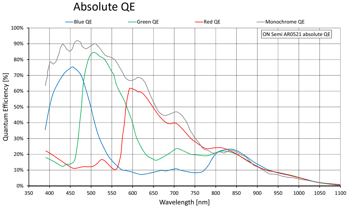
Figure 6: Alvium G5-500m/c (ON Semi AR0521) absolute QE
