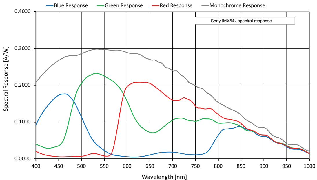
Figure 23: Alvium G5-2040m/c (Sony IMX541) spectral response
