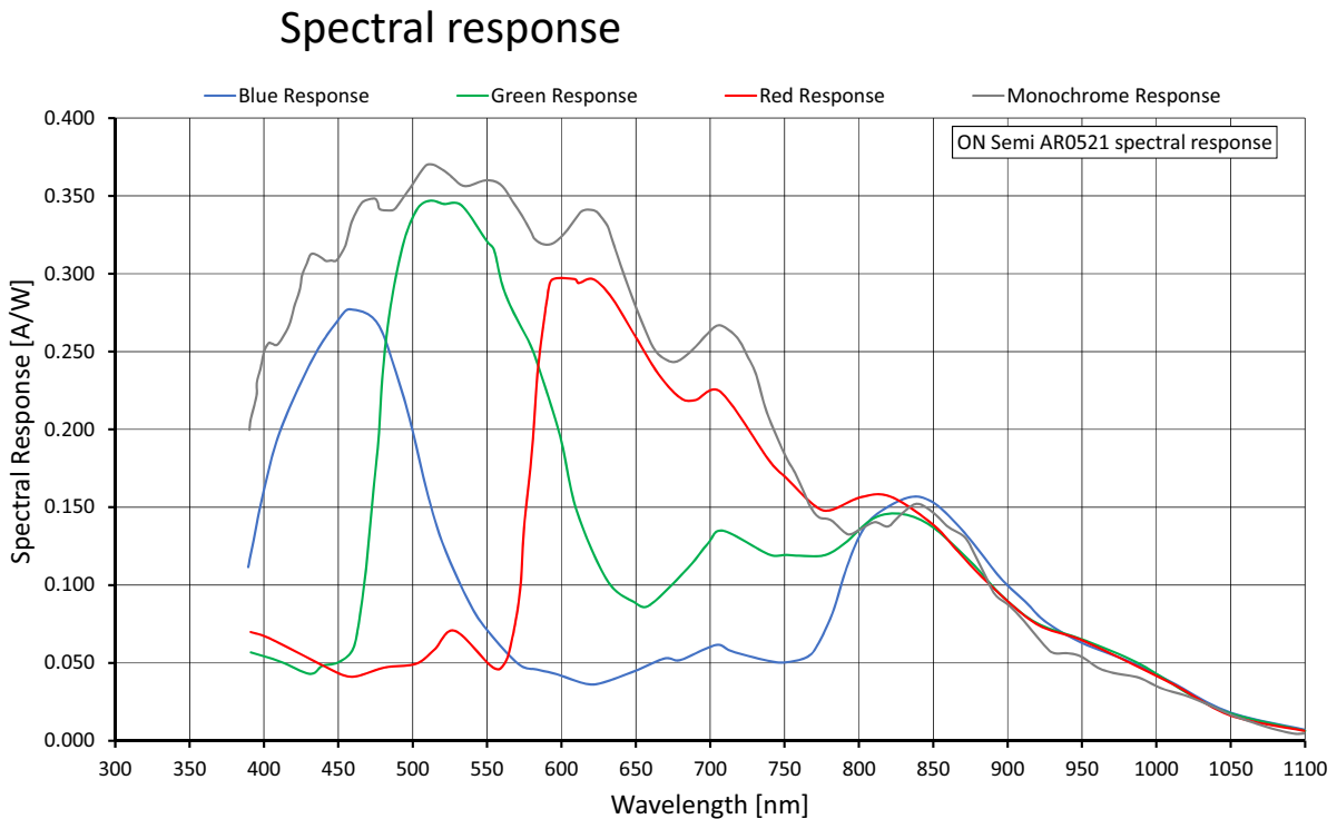
Figure 7: Alvium G5-500m/c (ON Semi AR0521) spectral response
