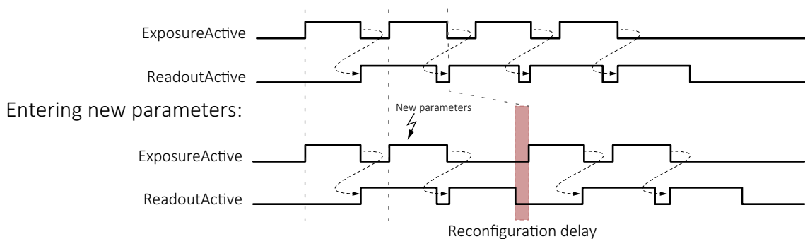
Figure 65: Delayed exposure due to parameter changes
