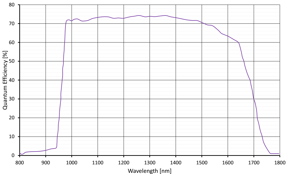
Figure 35: Goldeye CL-032 TEC1 absolute QE
