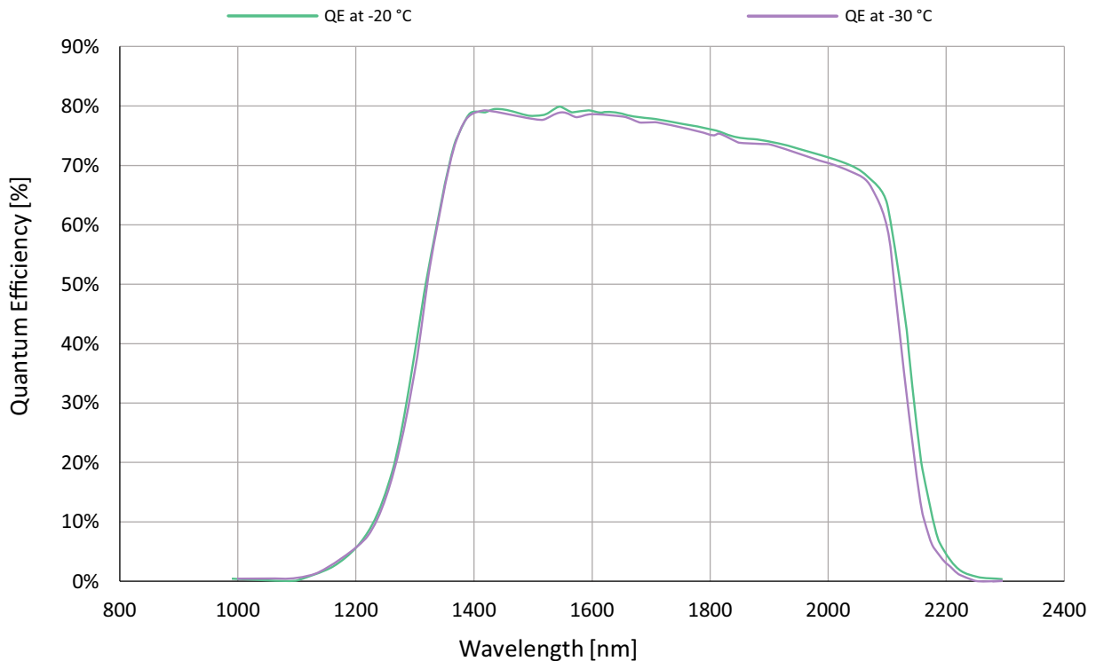
Figure 28: Goldeye G-034 XSWIR 2.2 TEC2 absolute QE
