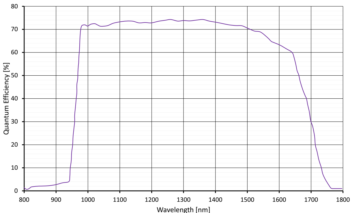
Figure 22: Goldeye G-032 TEC1 absolute QE
