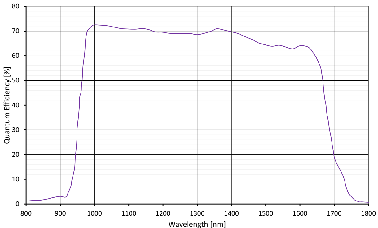
Figure 30: Goldeye CL-008 TEC1 absolute QE
