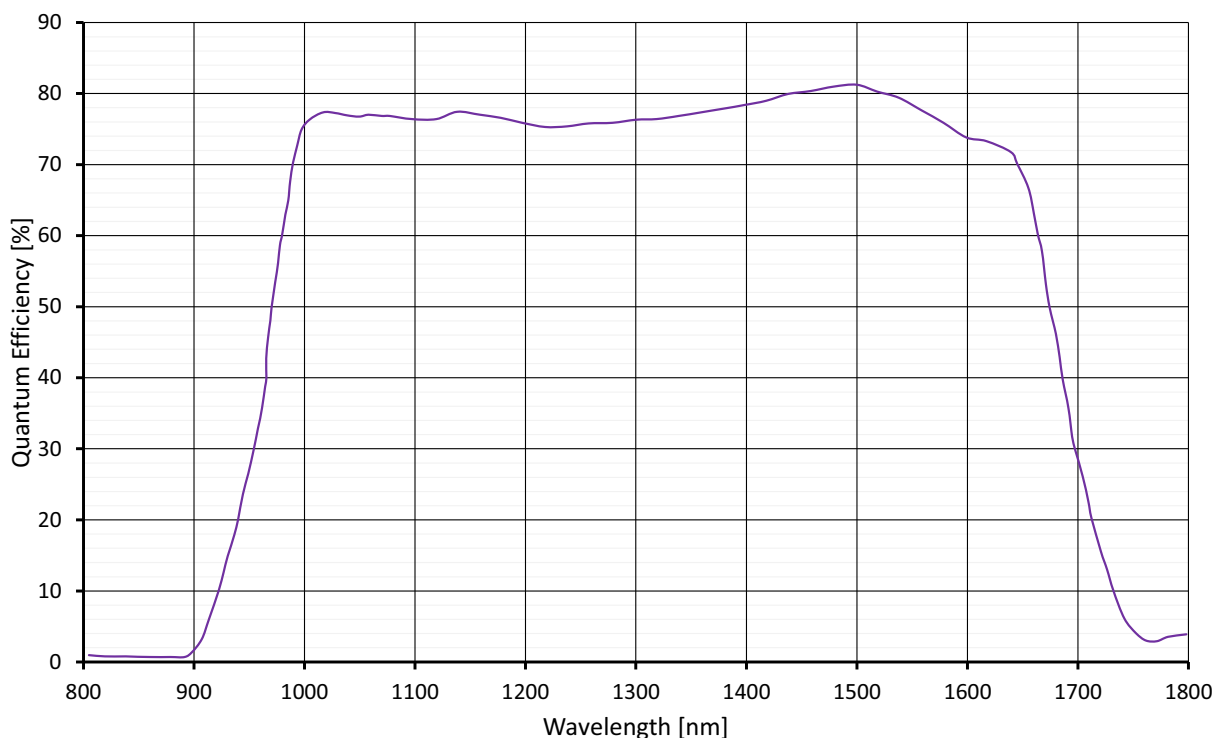
Figure 24: Goldeye G-033 TEC1 absolute QE
