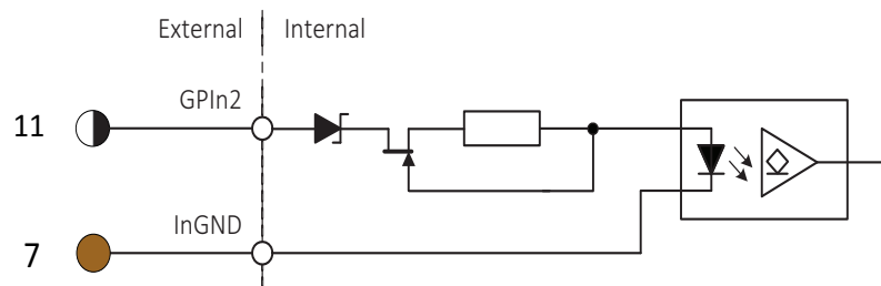
Figure 81: Goldeye G/CL isolated input block diagram
