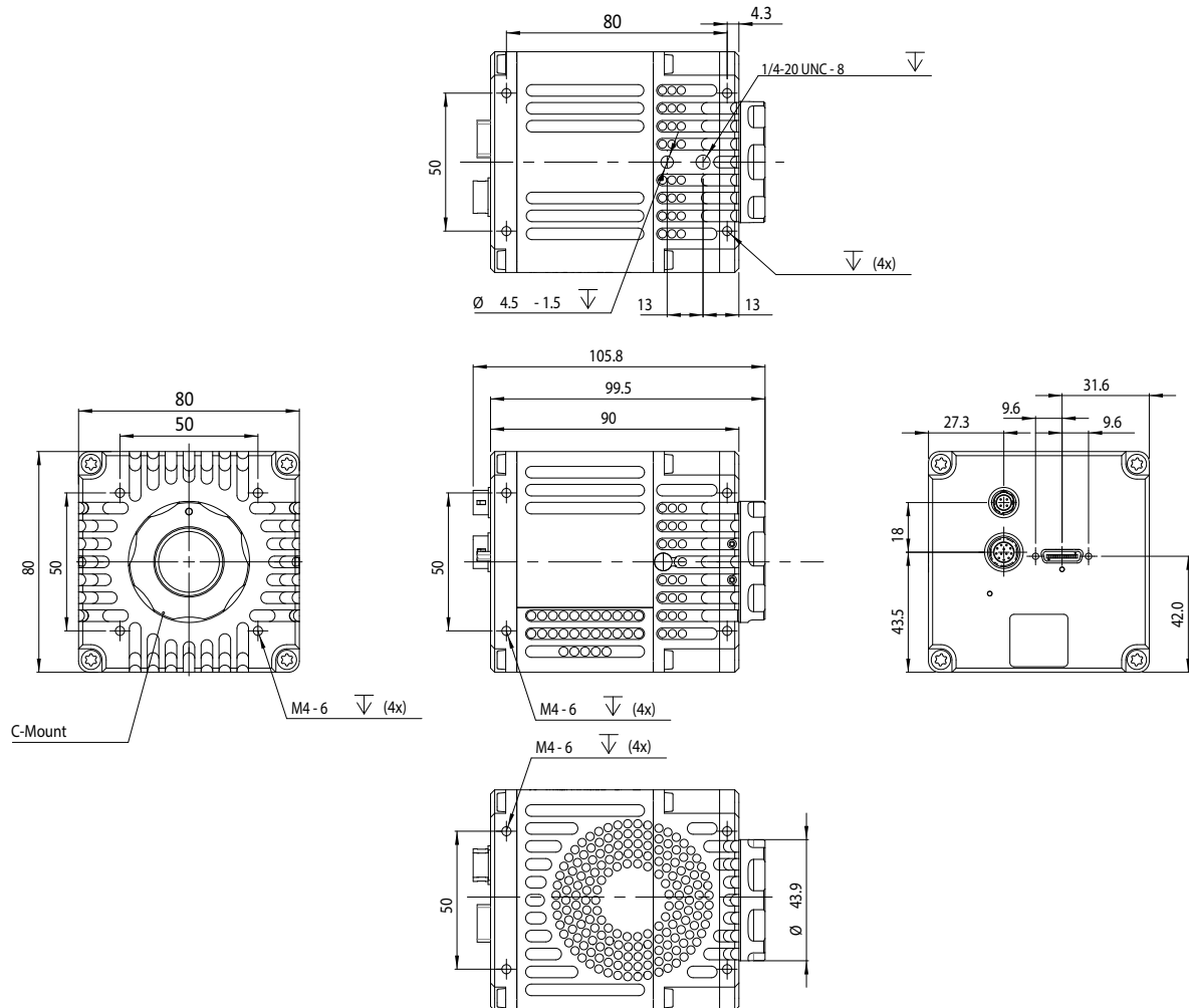
Figure 62: Goldeye CL Cool model dimensions with C-Mount lens adapter
