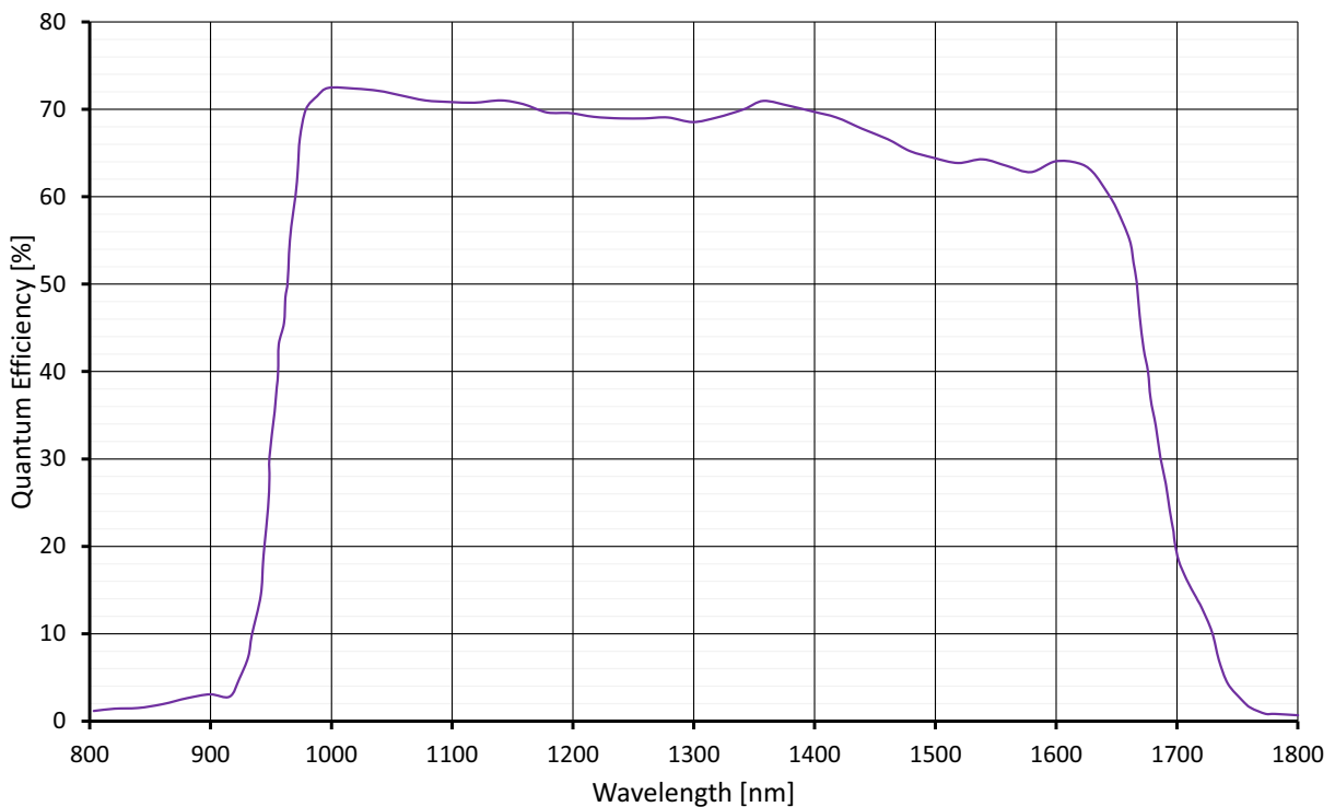
Figure 18: Goldeye G-008 Cool TEC1 absolute QE
