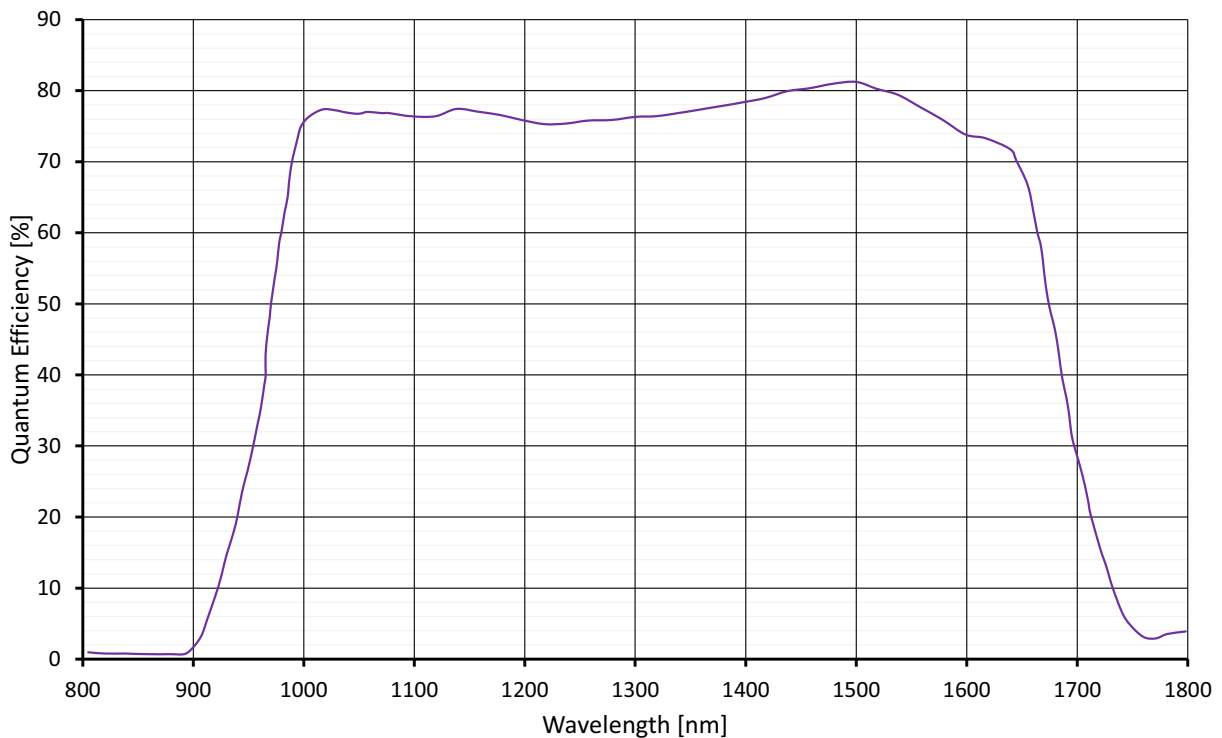
Figure 37: Goldeye CL-033 TEC1 absolute QE
