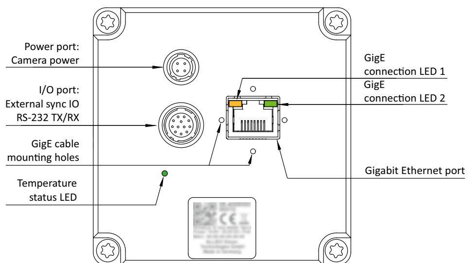
Figure 78: Connection ports and LEDs of Goldeye G-032 Cool and G-008 Cool
