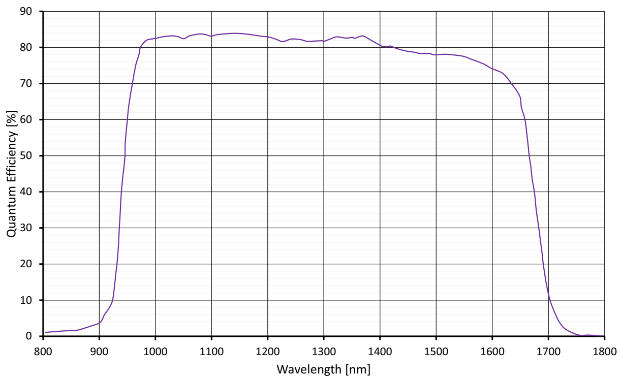
Figure 26: Goldeye G-034 TEC1 absolute QE
