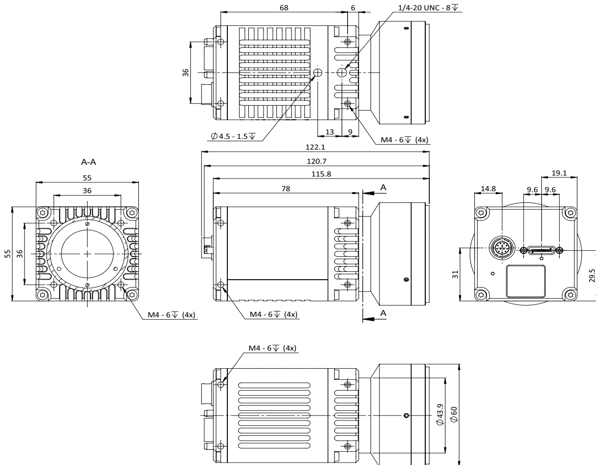
Figure 57: Goldeye CL dimensions with F-Mount lens adapter
