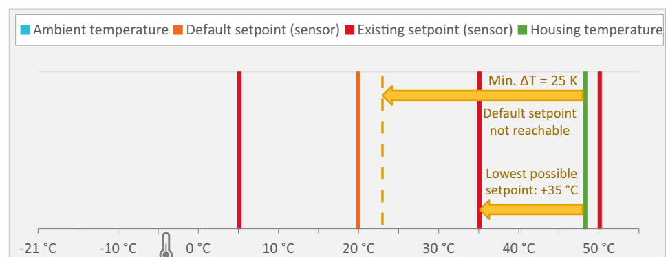
Figure 102: Cooling capabilities of Goldeye TEC1 models (example)
