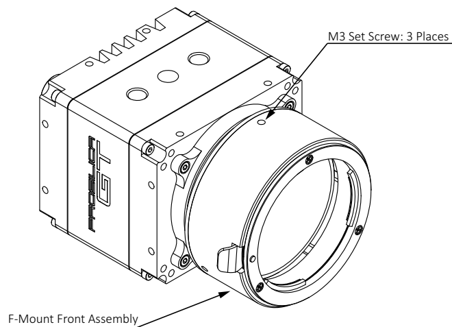
Figure 86: Prosilica GT Large Format with F-Mount isometric view
