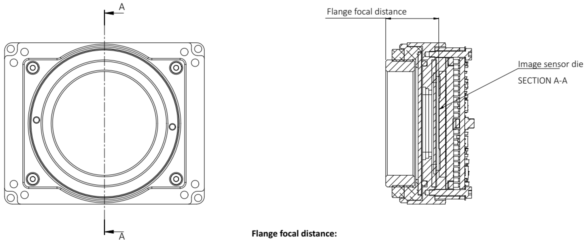
Figure 91: TFL-Mount flange focal distance
