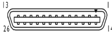
Figure 7. MDR26 Camera Link Connector
