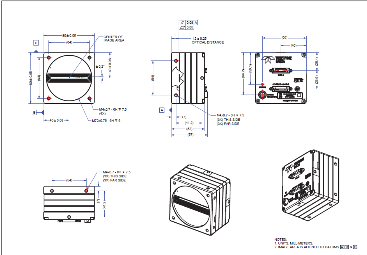
Figure 4: Camera Mechanical
