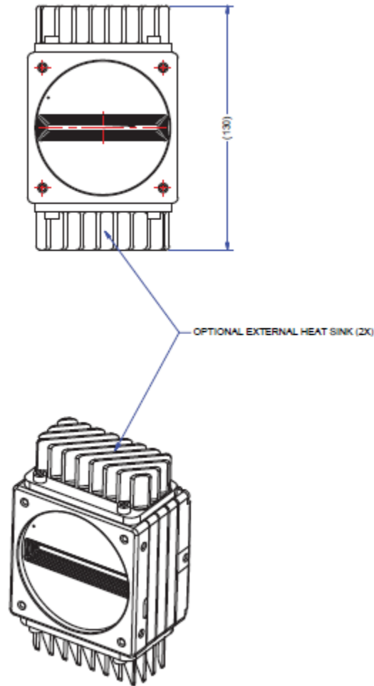
Figure 5: Camera Mechanical with External Heat Sink
