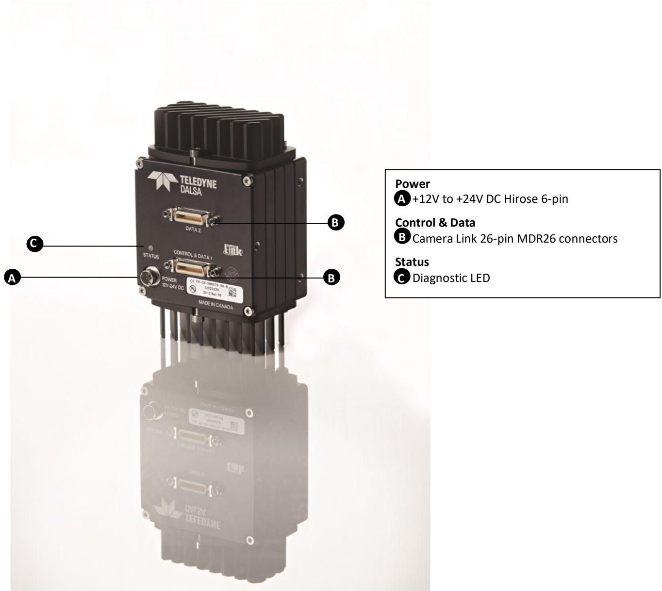
Figure 6: Input and Output, Trigger, and Power Connectors
