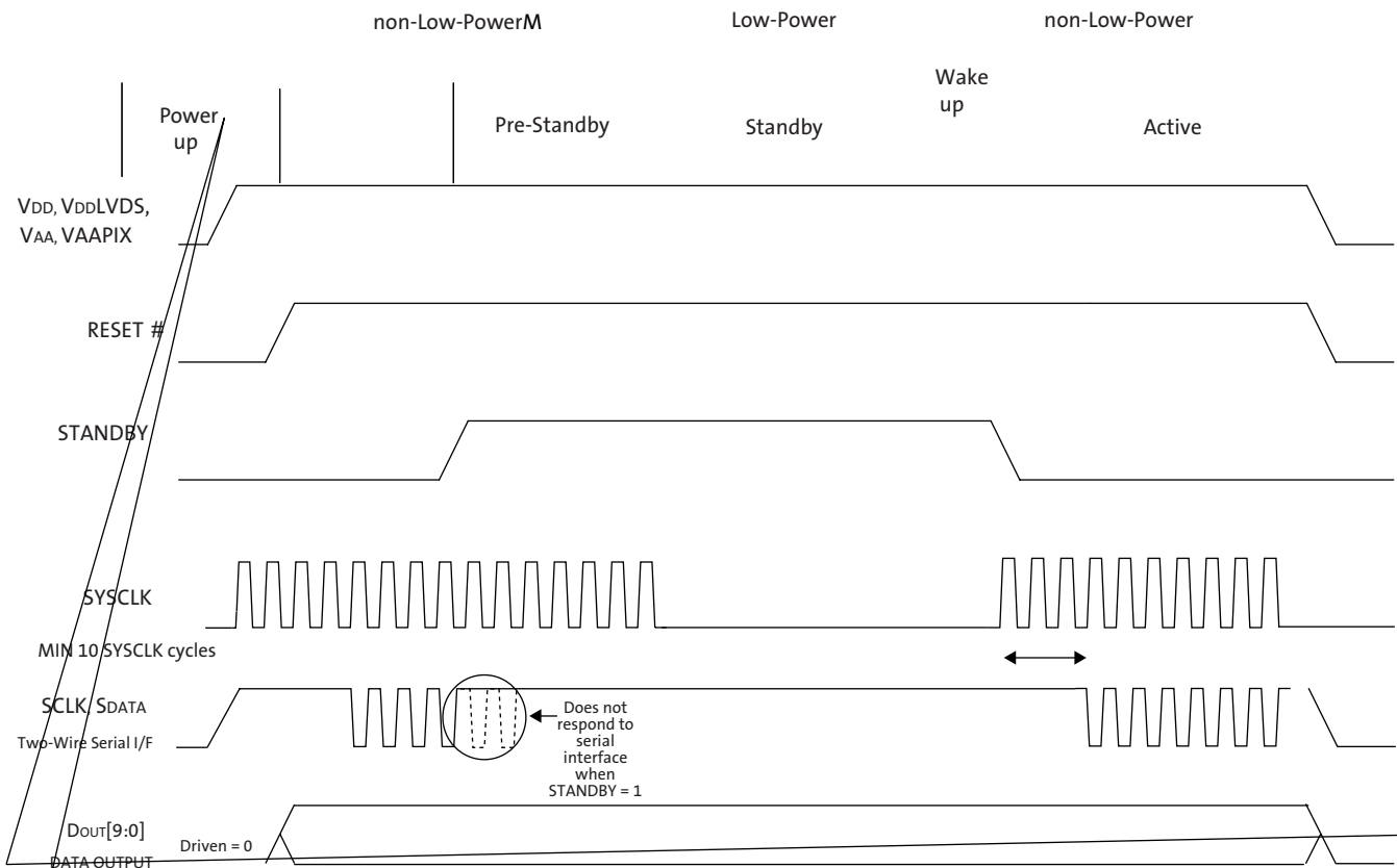
Figure 49: Power-up, Reset, Clock and Standby Sequence
