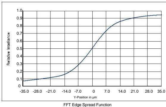
12X Zoom @ 7X High Mag 2MP Sensor – 0.79 \mu\text{m} / pixel 1.55mm FOV – 1.28mm 2 Area
