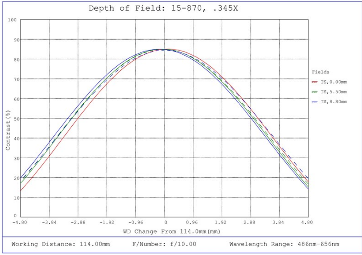
#15-870, 0.345X CobaltTTL Telecentric Lens, Depth of Field Plot, 114mm Working Distance, f10
