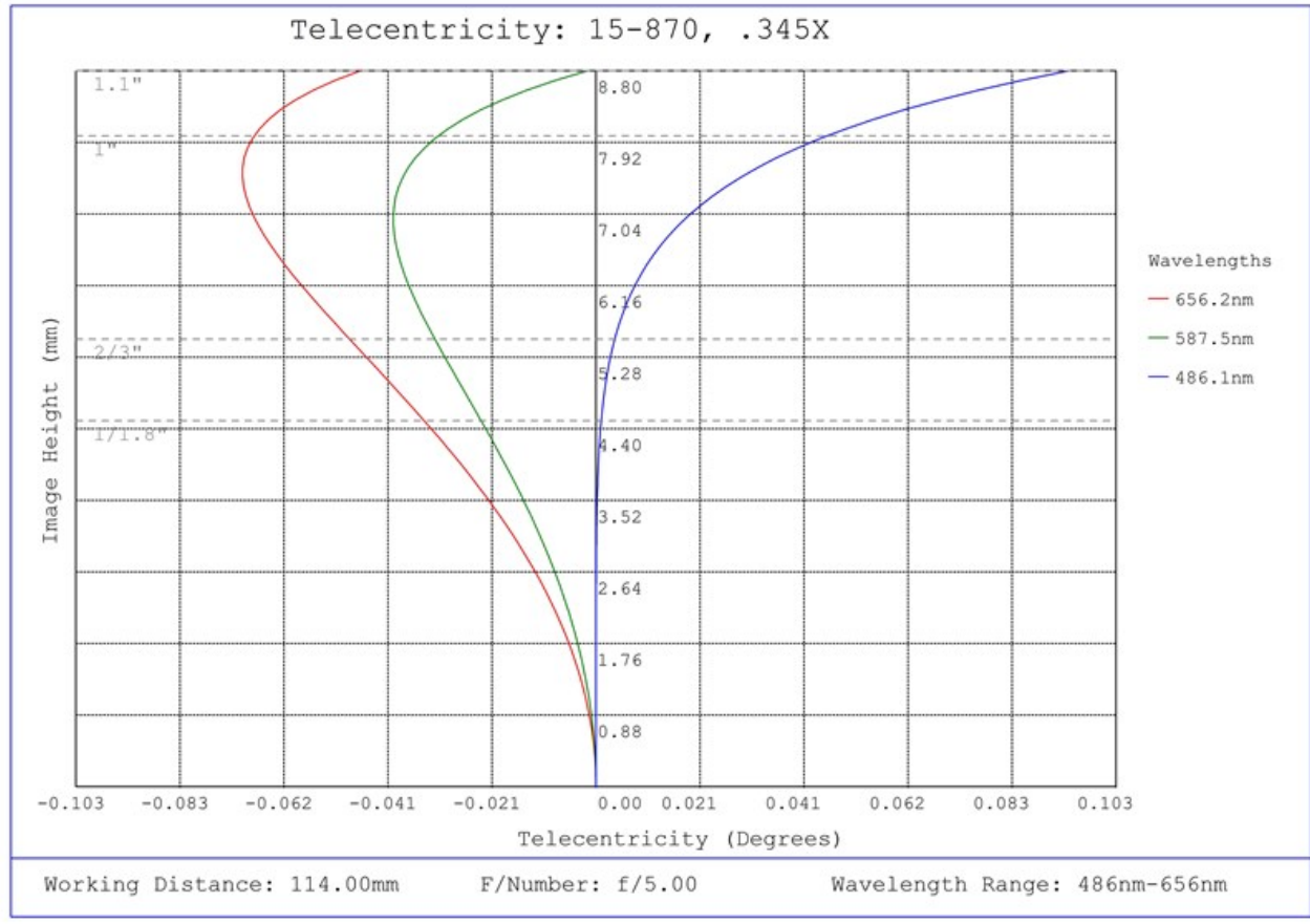
#15-870, 0.345X CobaltTL Telecentric Lens, Telecentricity Plot
