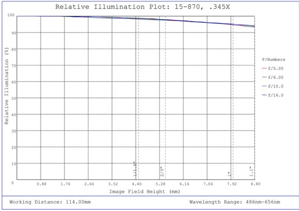
#15-870, 0.345X CobaltTL Telecentric Lens, Relative Illumination Plot
