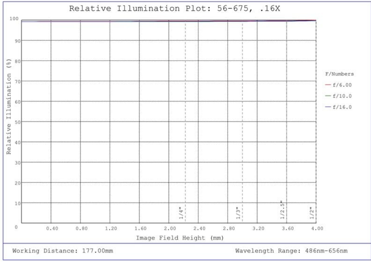
#56-675, 0.16X SilverTL™ Telecentric Lens, Relative Illumination Plot
