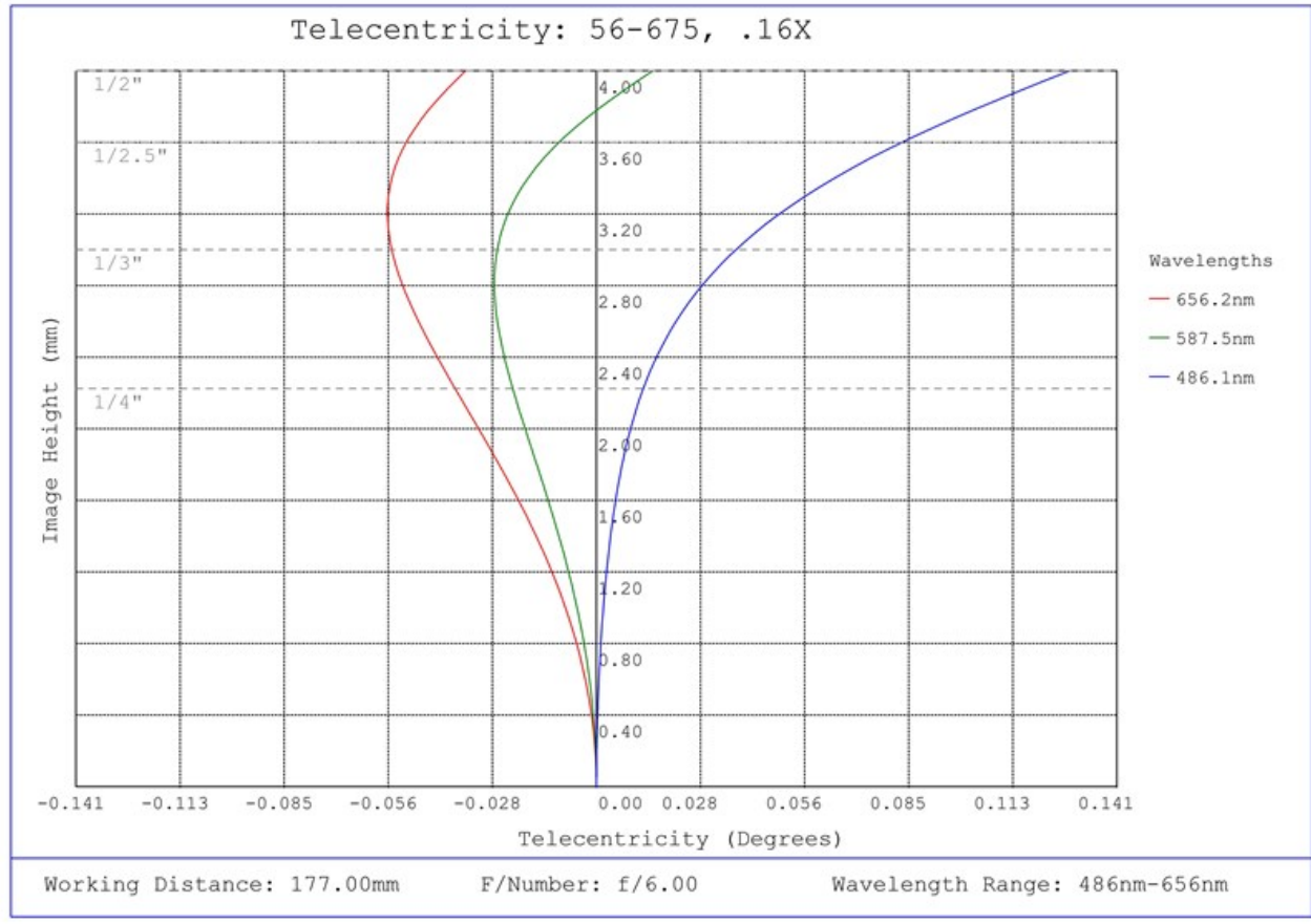
#56-675, 0.16X SilverTL™ Telecentric Lens, Telecentricity Plot
