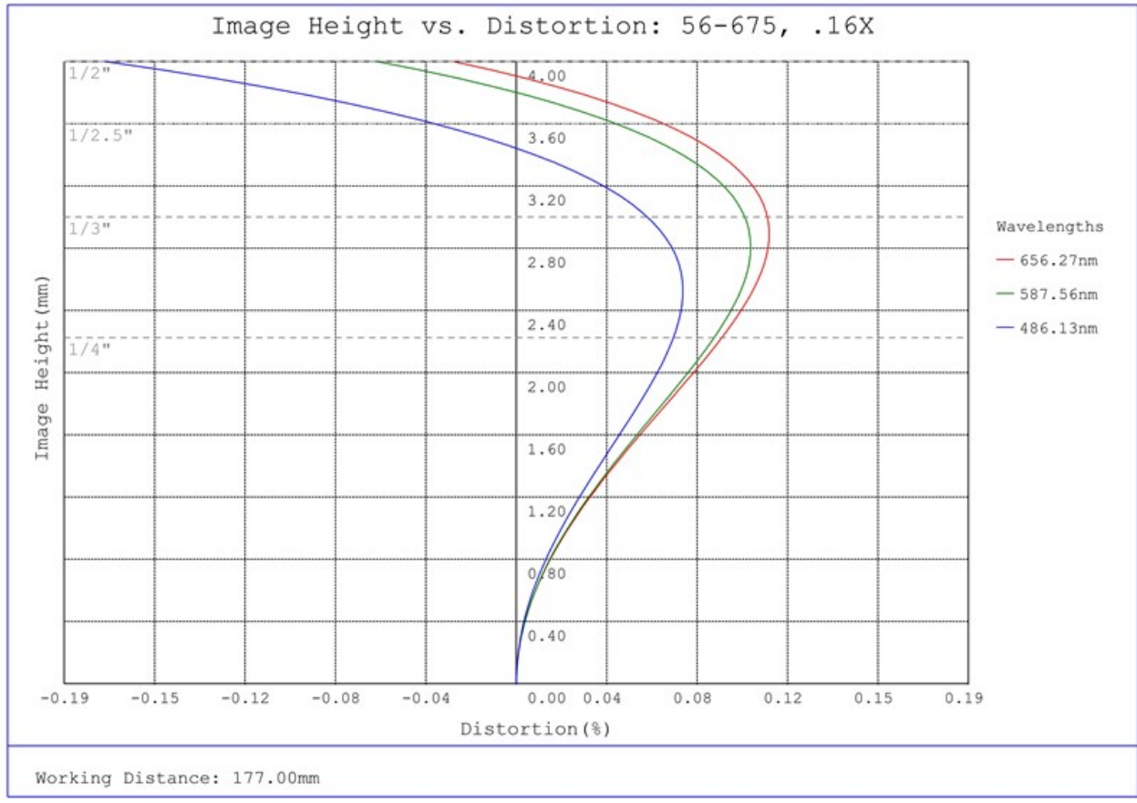
#56-675, 0.16X SilverTL™ Telecentric Lens, Distortion Plot
