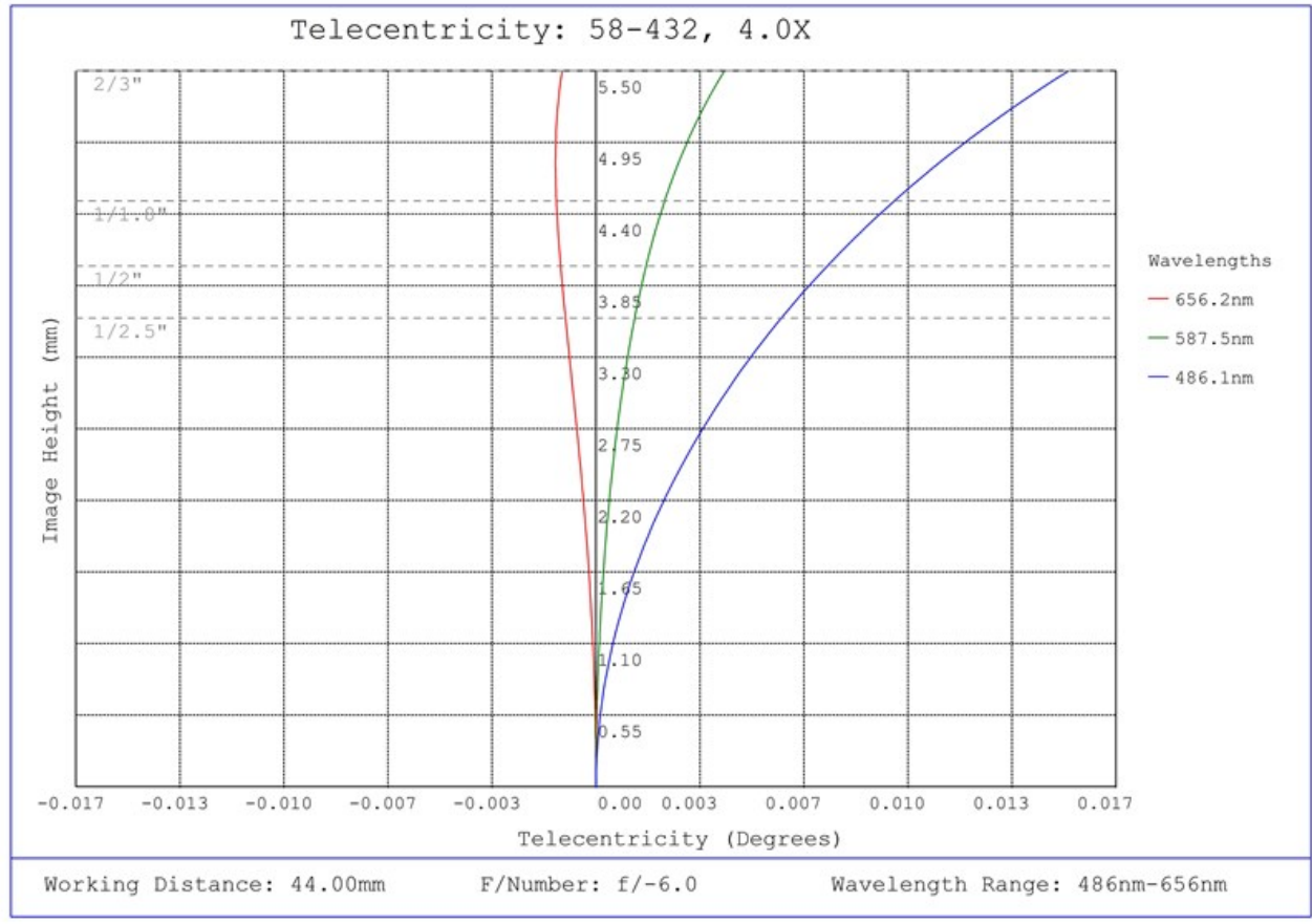
#58-432, 4.0X SilverTL™ Telecentric Lens, Telecentricity Plot
