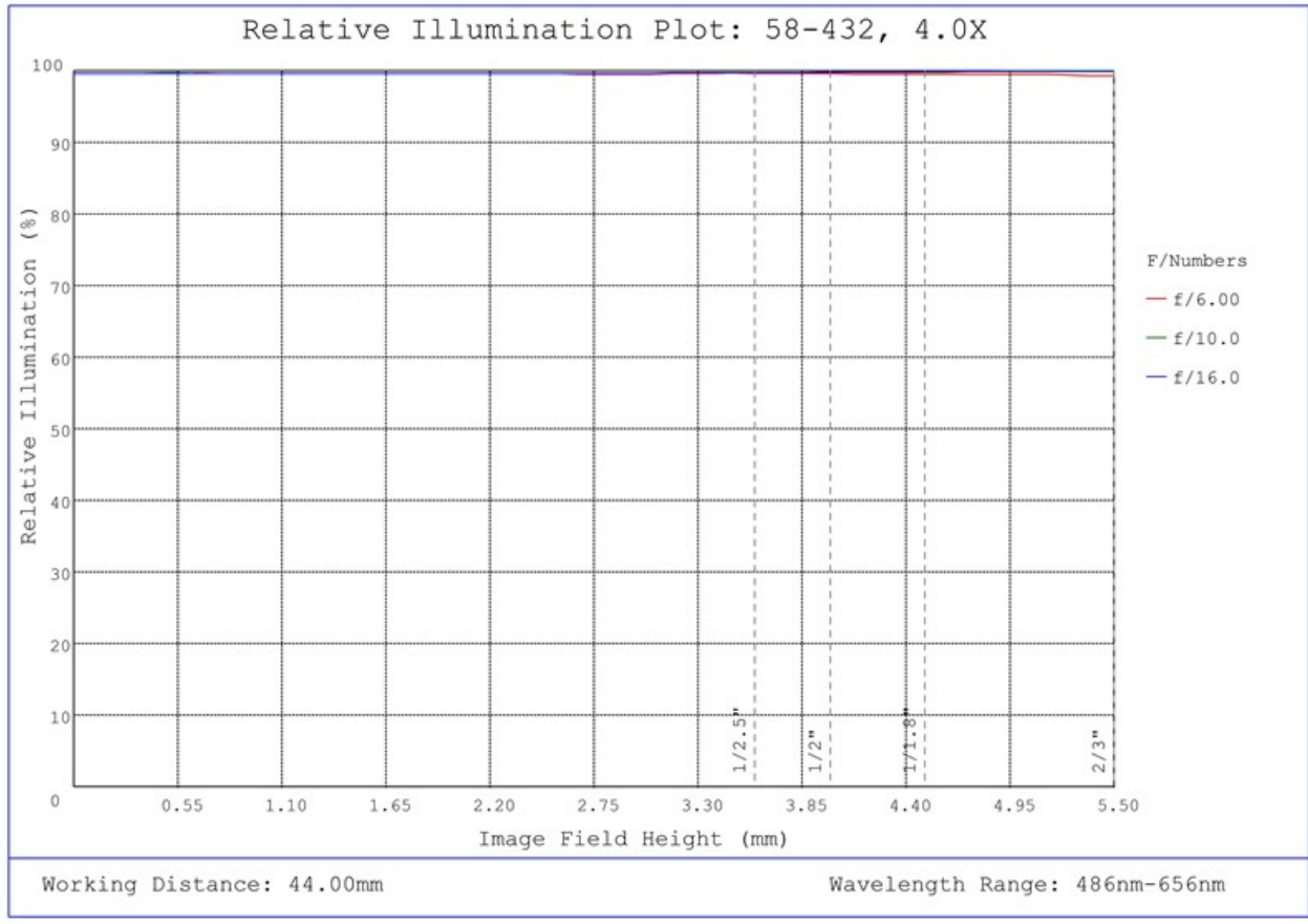
#58-432, 4.0X SilverTL™ Telecentric Lens, Relative Illumination Plot
