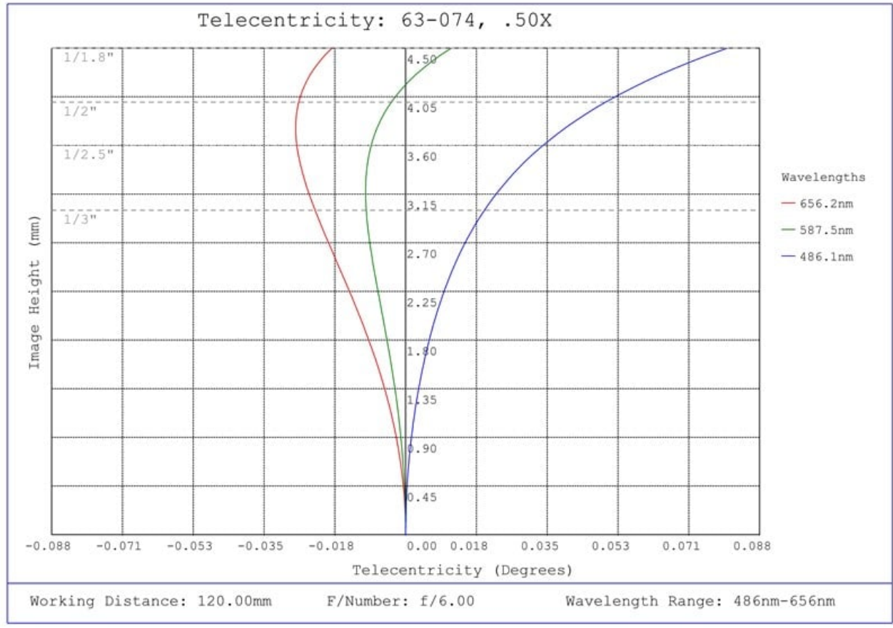
#63-074, 0.50X SilverTL™ Telecentric Lens, Telecentricity Plot
