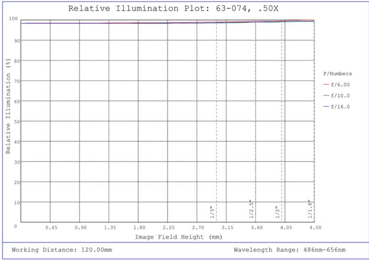
#63-074, 0.50X SilverTL™ Telecentric Lens, Relative Illumination Plot
