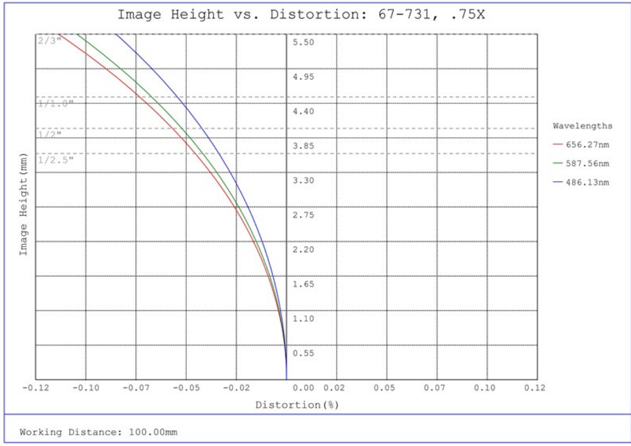
#67-731, 0.75X SilverTL™ Telecentric Lens, Distortion Plot
