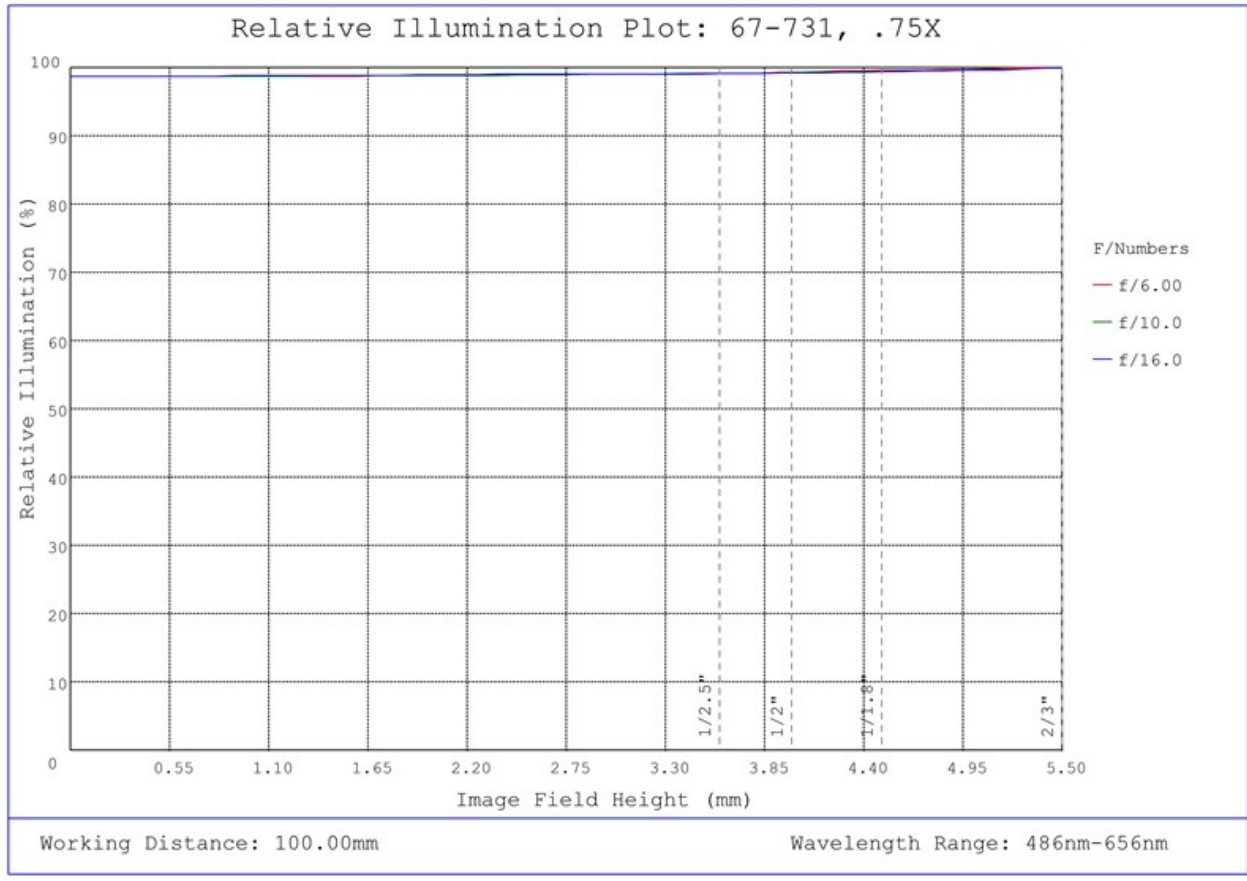
#67-731, 0.75X SilverTL™ Telecentric Lens, Relative Illumination Plot
