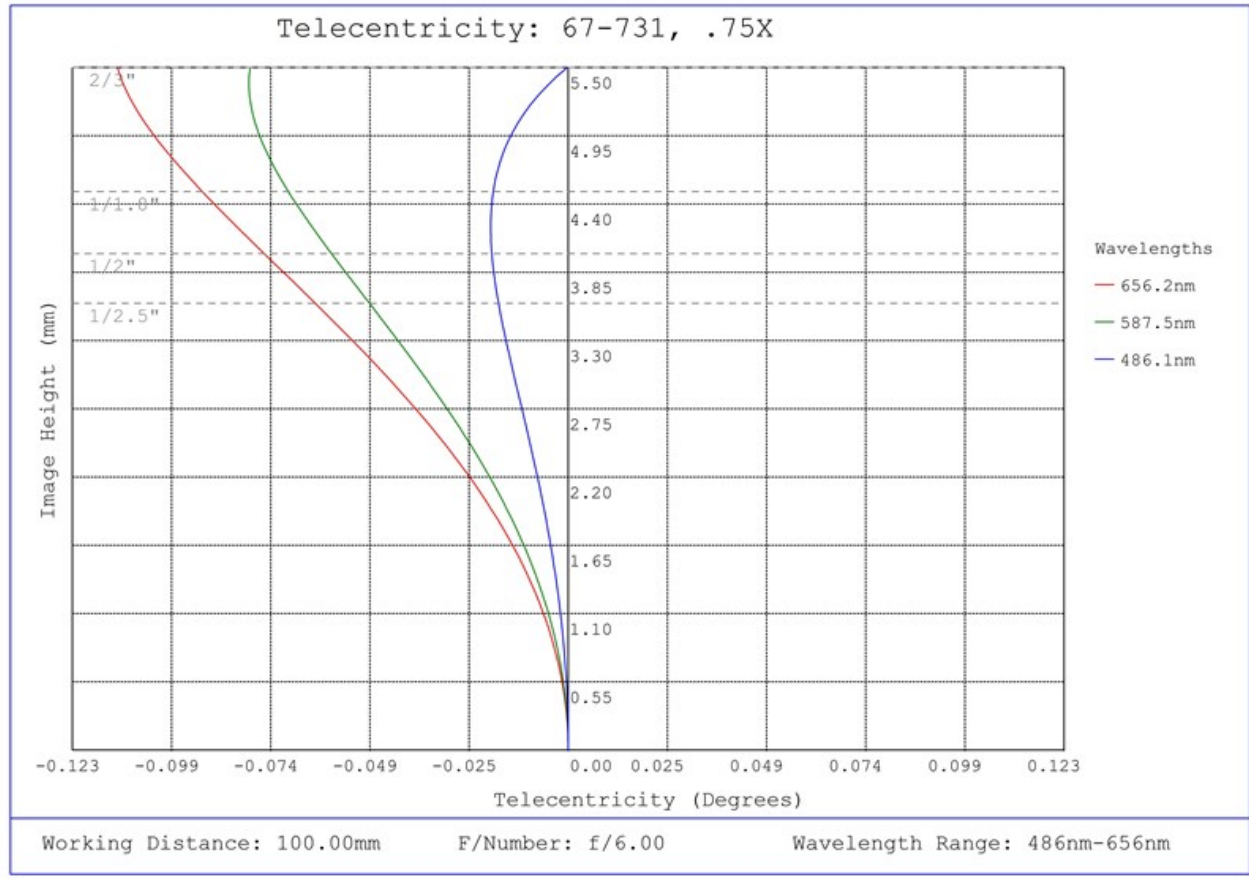
#67-731, 0.75X SilverTL™ Telecentric Lens, Telecentricity Plot
