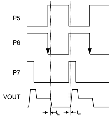
Figure 18: Pixel Timing Detail
