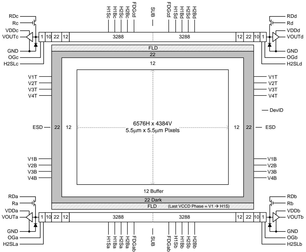
Figure 1: Block Diagram
