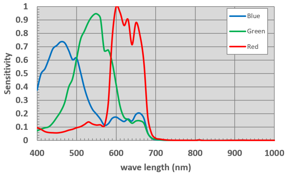
SW-4005 Sensitivity
