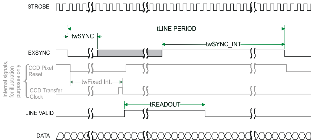
Figure 6. Spyder2 Fixed (Programmed) Integration Timing with External EXSYNC
