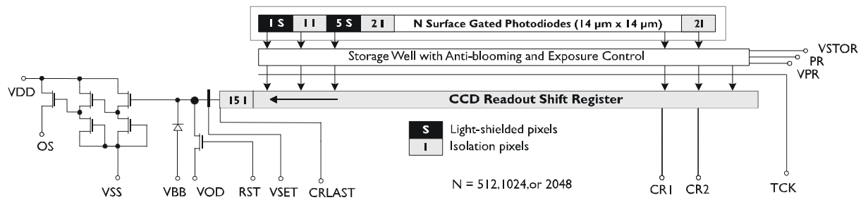
Figure 1. IL-P3 Image Sensor Block Diagram
