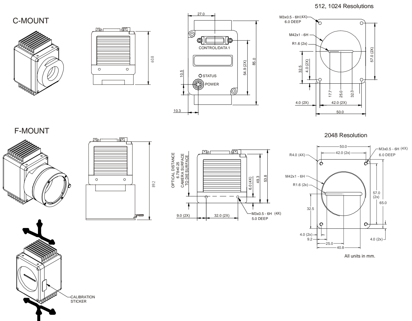
Figure 9. Spyder2 Mechanical Interface
