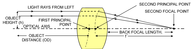
Figure 10. Primary Points in a Lens System
