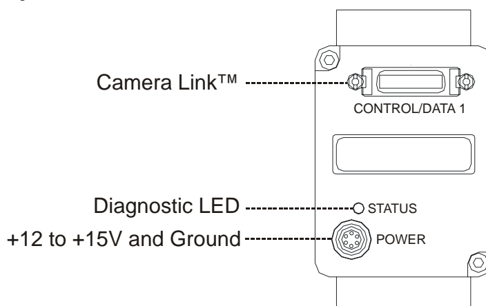
Figure 3: Camera Inputs/Outputs
