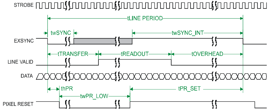
Figure 5. Spyder2 Overview Timing Showing Input and Output Relationships
