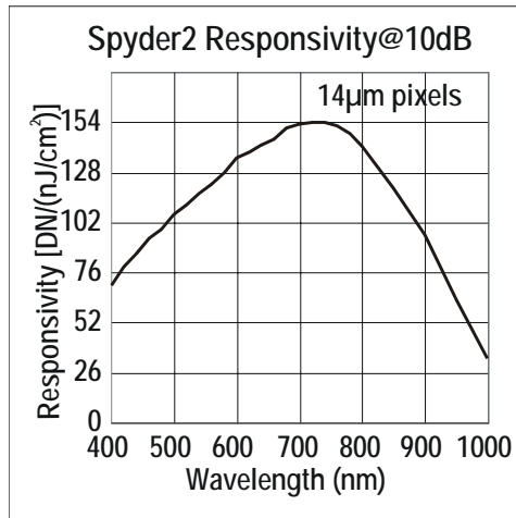
Figure 2: Spyder2 Responsivity
