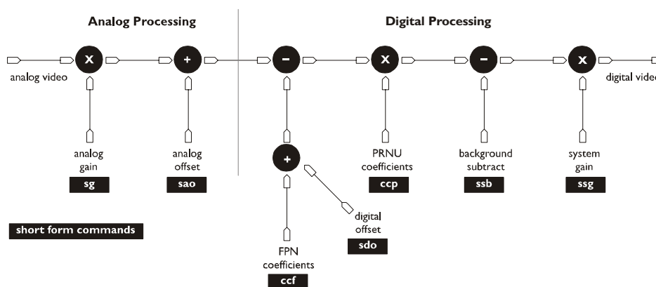
Figure 7: Camera Processing Chain
