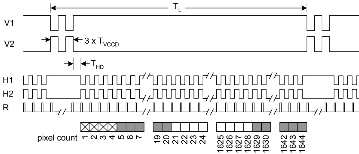
Figure 23: Line Timing Vertical Binning by 2
