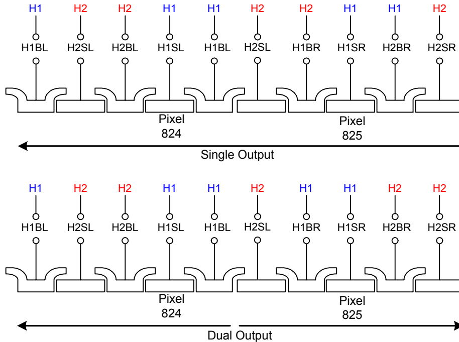
Figure 5: Horizontal Register
