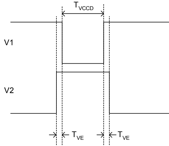
Figure 26: Line Timing Edge Alignment
