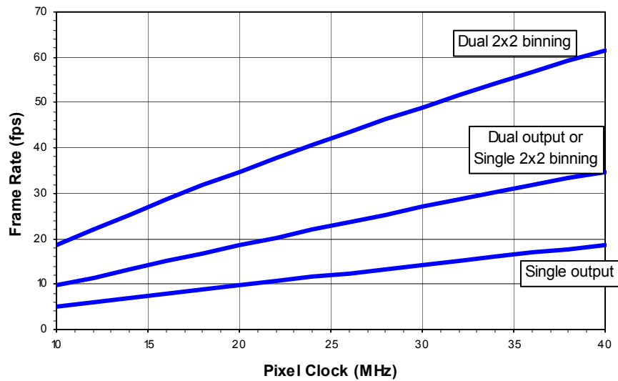
Figure 9: Frame Rates
