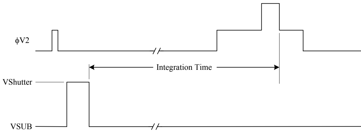
Figure 31: Integration Time Definition
