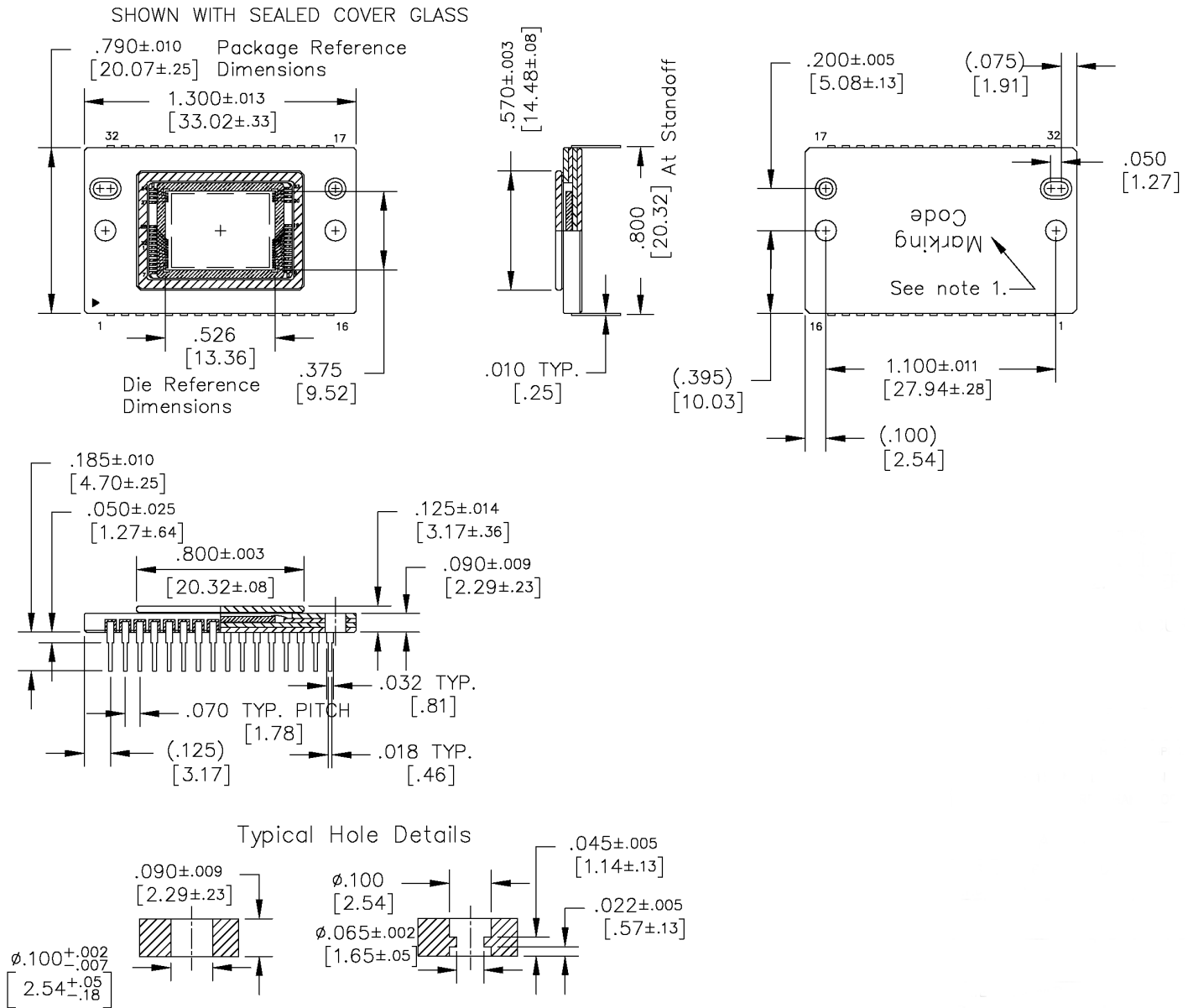
Figure 32: Completed Assembly (1 of 2)
