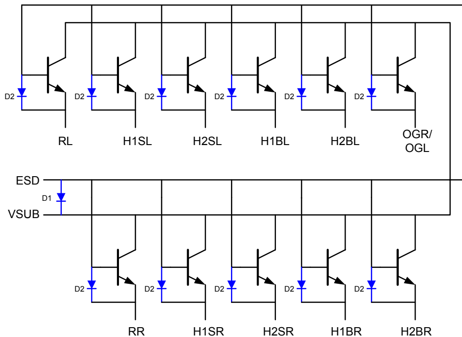
Figure 7: ESD Protection
