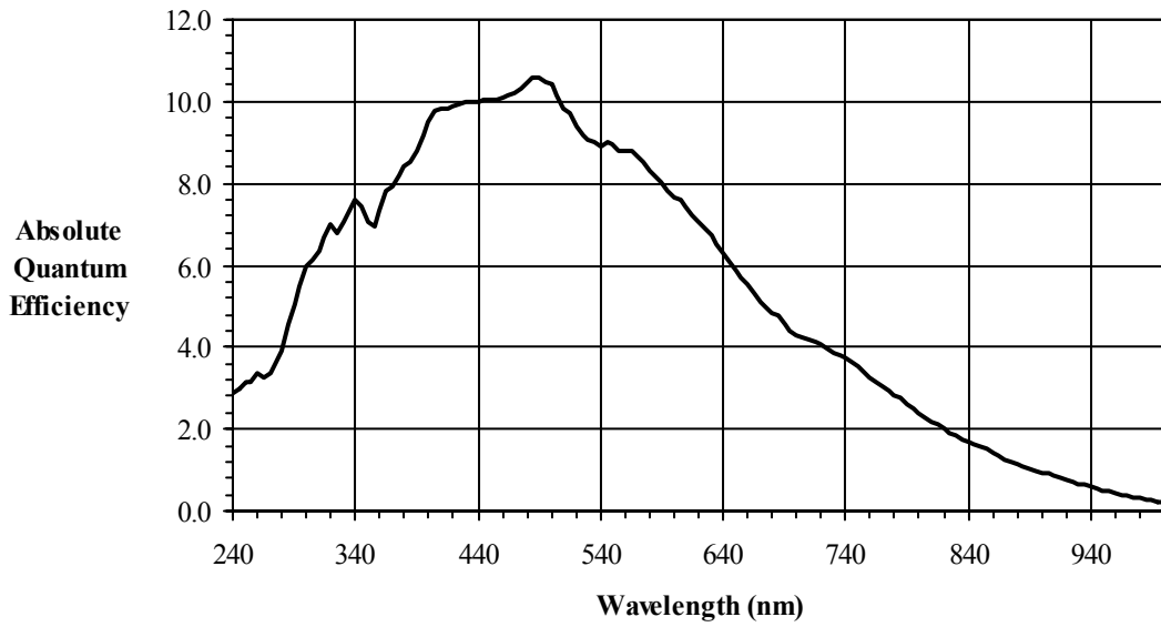
Figure 12: Ultraviolet Quantum Efficiency (without coverglass)
