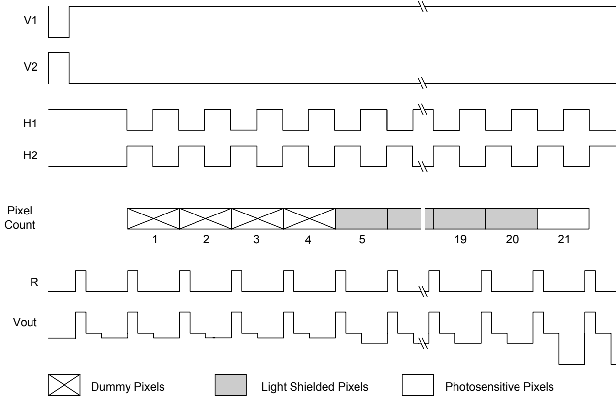
Figure 27: Pixel Timing
