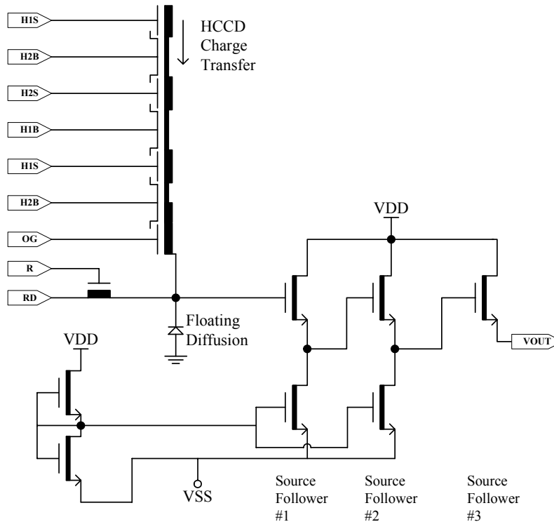
Figure 6: Output Architecture
