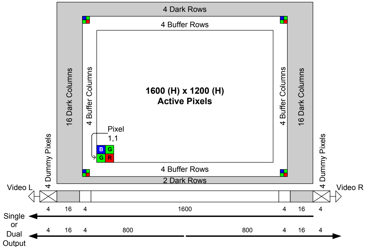
Figure 1: Sensor Architecture
