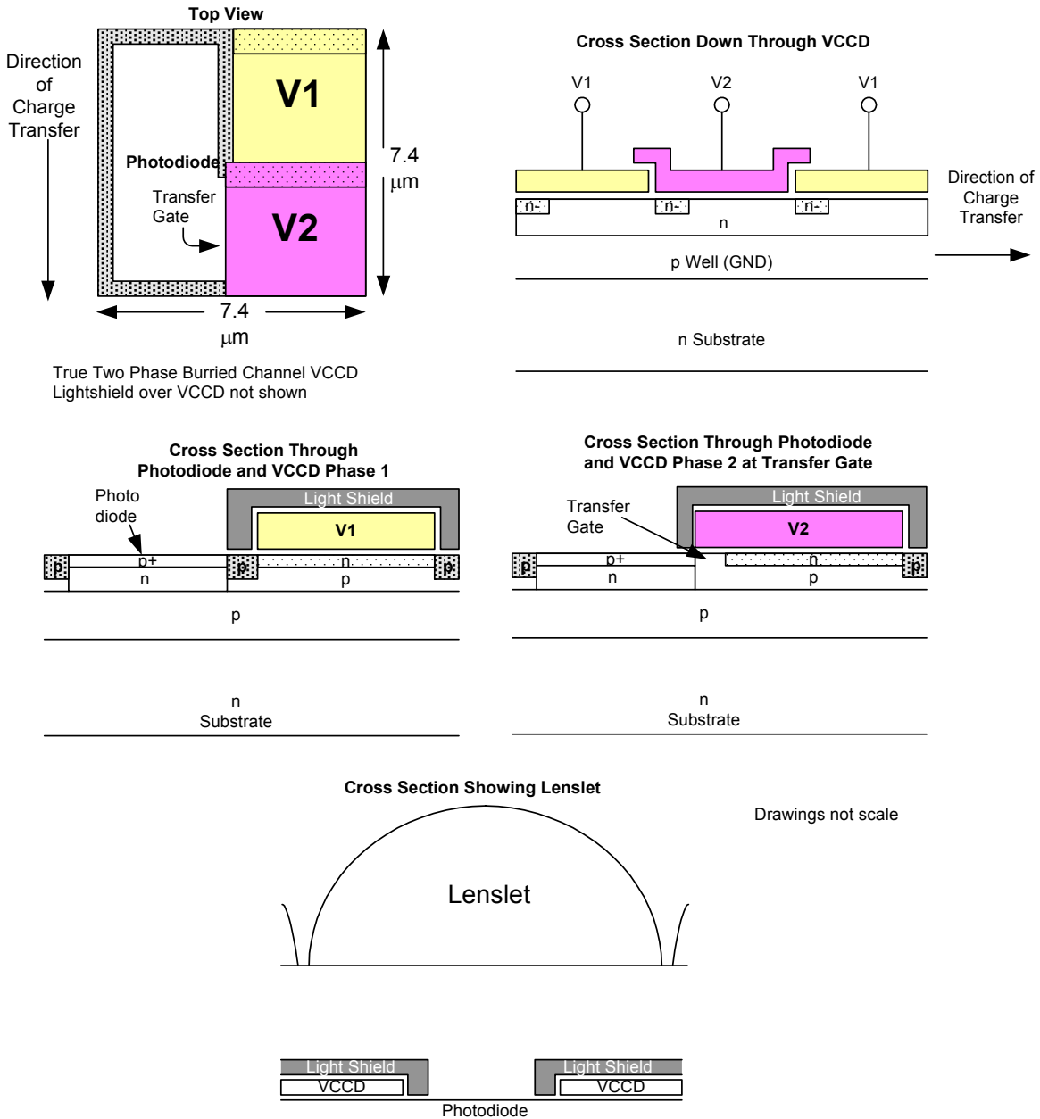
Figure 2: Pixel Architecture
