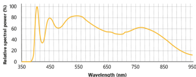
Spectral distribution graph of proprietary CCS LED technology used in the Hyper Spectral Range . These LEDs have continuous and tunable wide-band spectrums and can be adapted to any form factor, for better performance and cost benefits compared to traditional MSI/HSI solutions like halogen.
