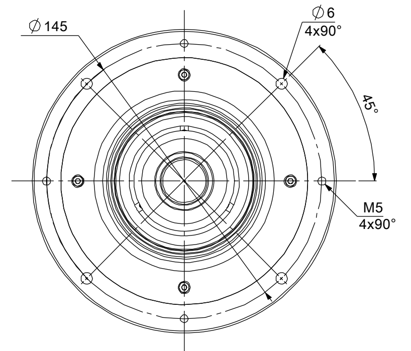
MOUNTING PORTION DETAIL VIEW
